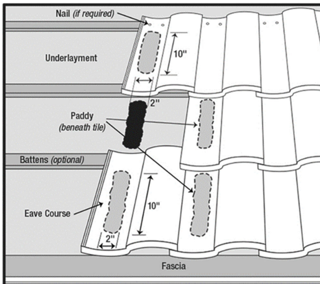
High Profile Tile – Large Paddy
